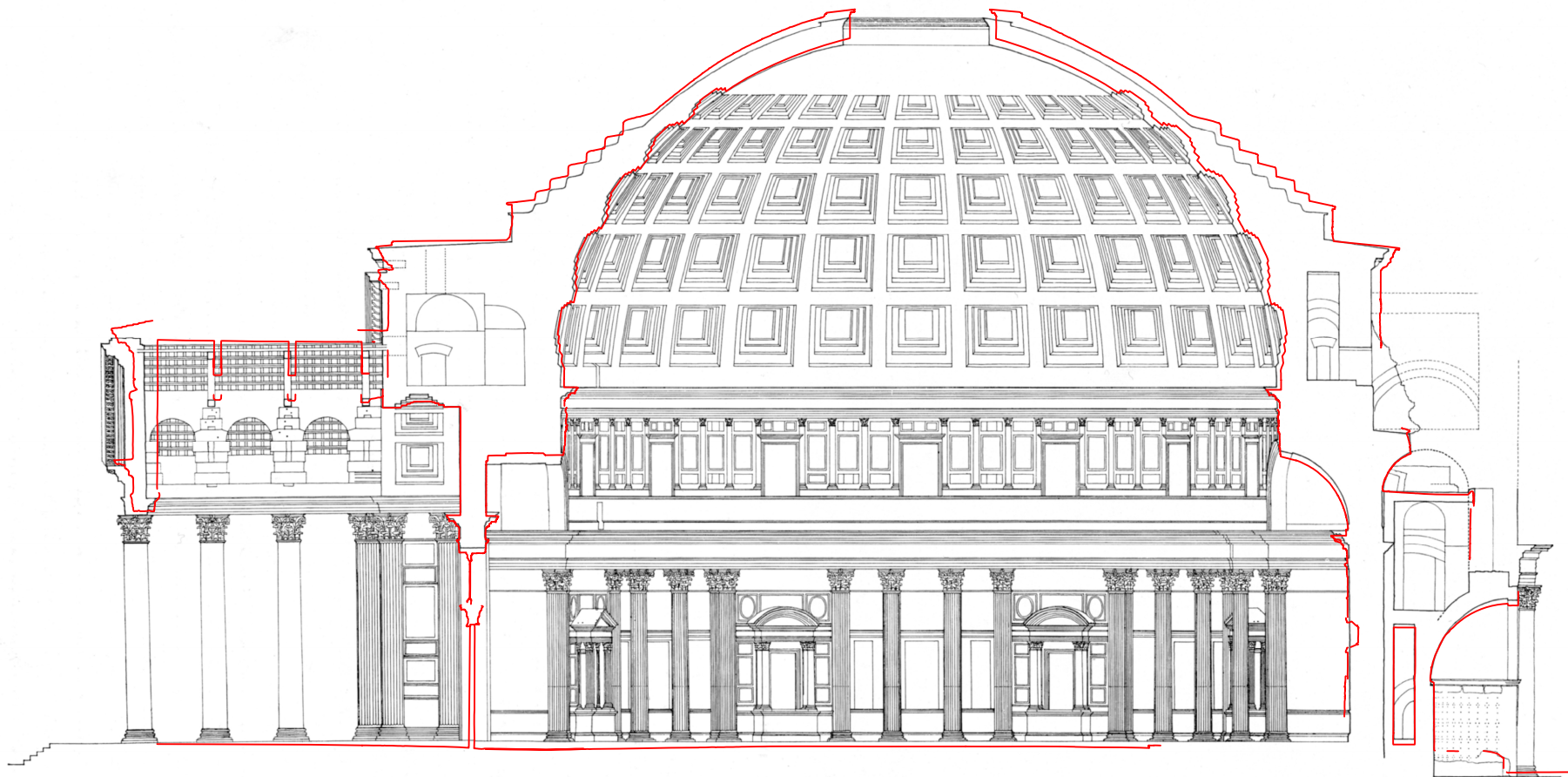
FIG. 105. Pantheon: Longitudinal section along the main axis 1:400.
