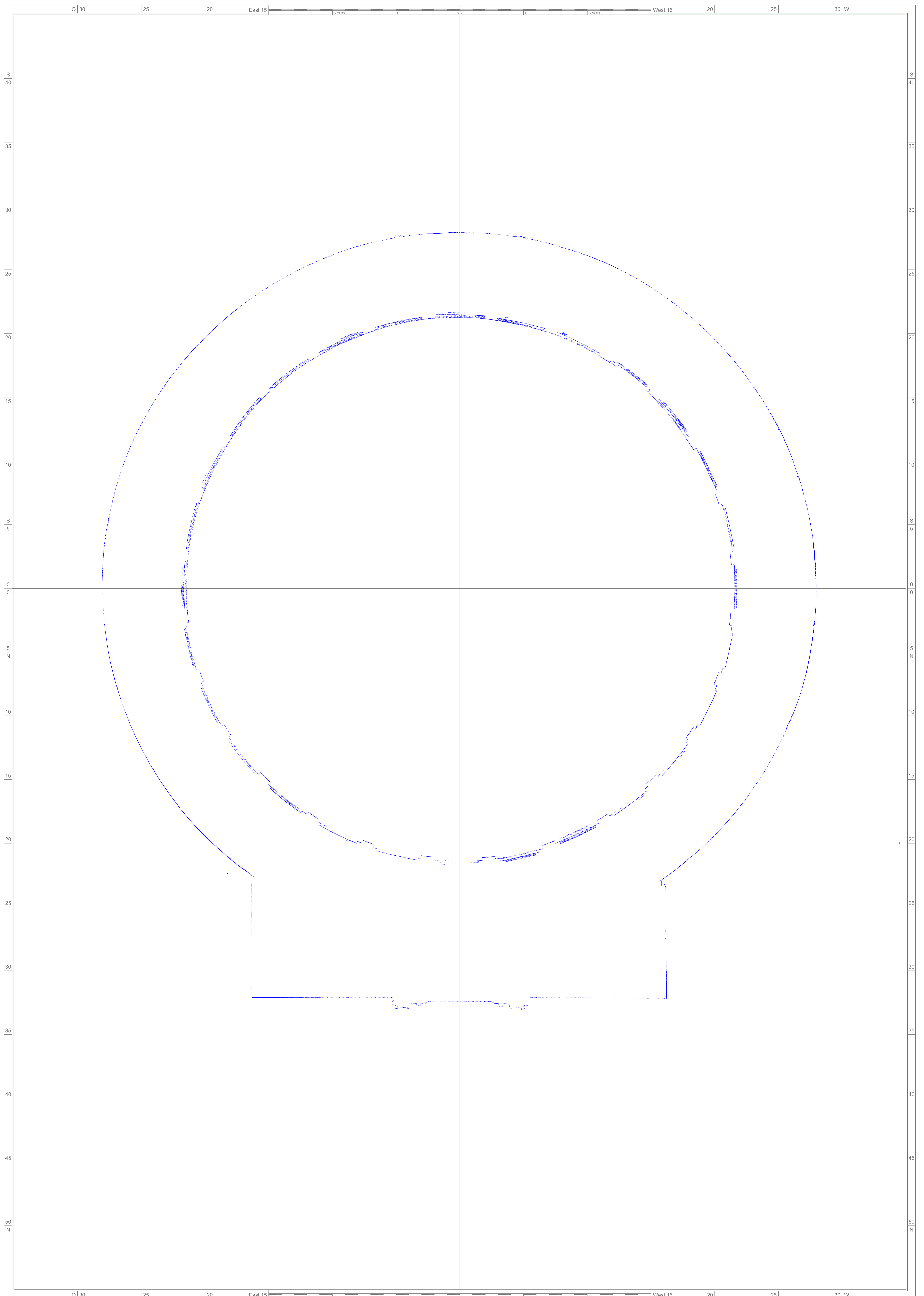
Section 27 (27 meter above z=0, slice thickness 0,10 m)
