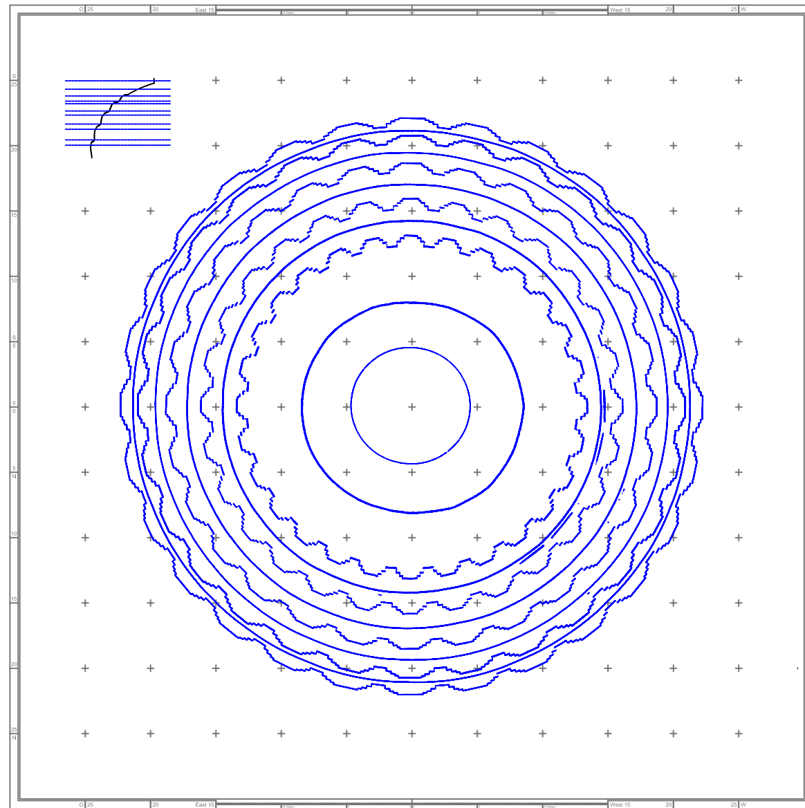
Trace plans superimposed: showing sections between each coffer row and dome shell (slice thickness 0,05 m)
