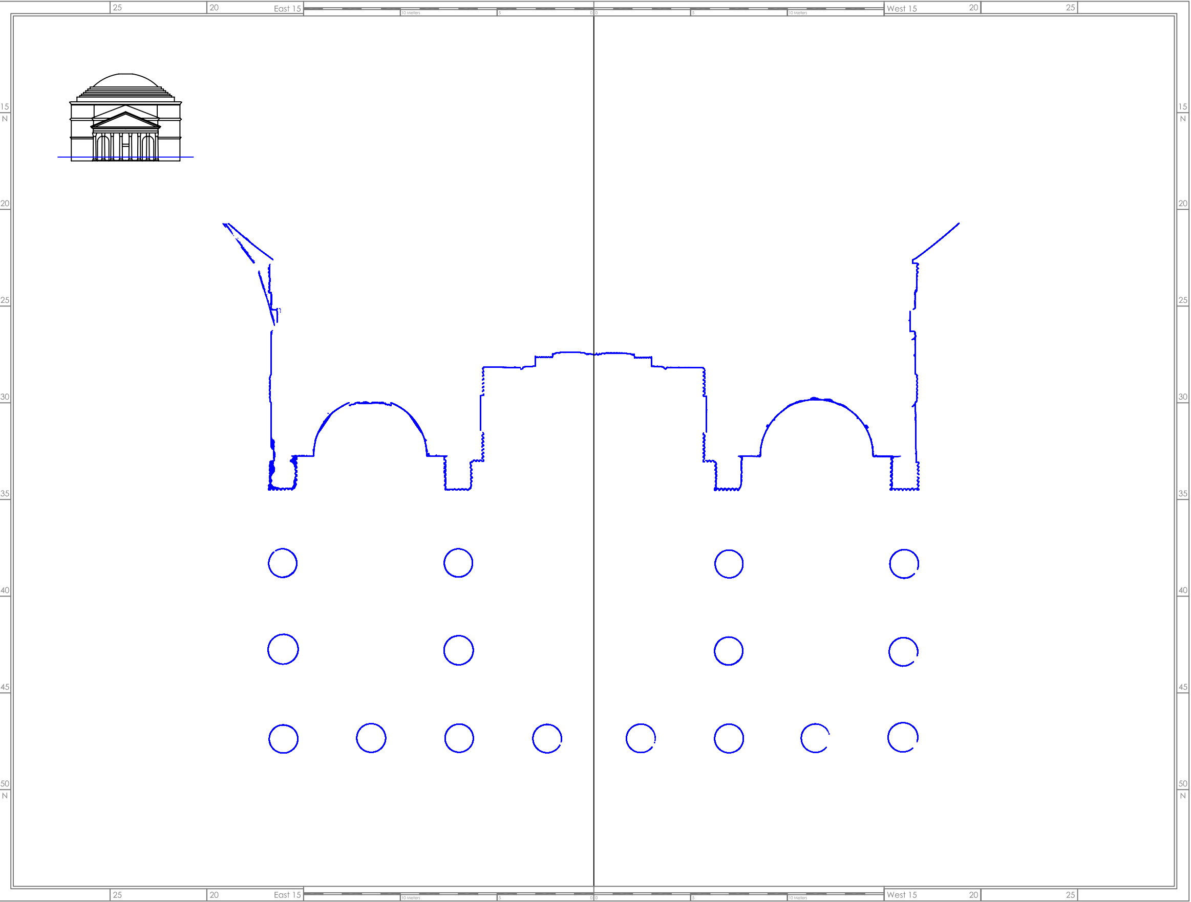
Section of Porticus (level 2 m above ground floor, slice thickness 0,05 m)
